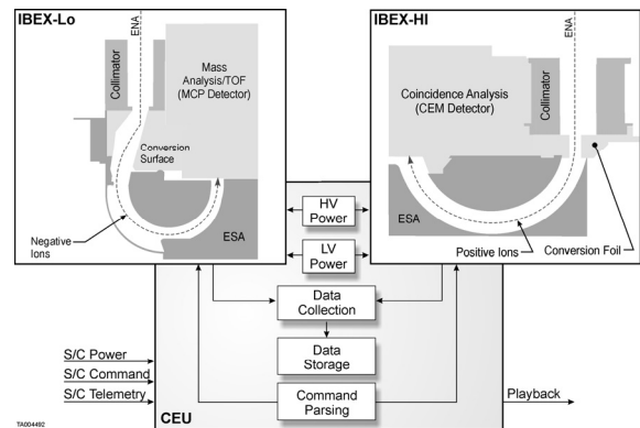
Figure 3. Schematic diagram of the IBEX payload, which consists of two large-aperture sensors, IBEX-Lo ( \sim 10\text{eV}-2\text{keV} ) and IBEX-Hi ( \sim 300\text{eV}-6\text{keV} ), and a Combined Electronics Unit.
