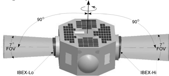
Figure 2. IBEX's simple sun-pointed spinning spacecraft. The ENA sensors look off sideways and sweep out swaths of the sky each spacecraft spin.
